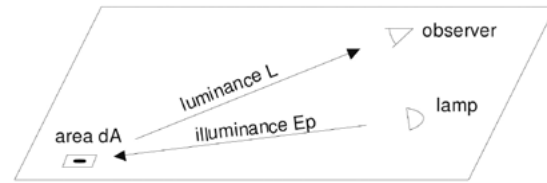
Fig 2. the coefficient of retroreflected luminance(Sorensen, 2011)
