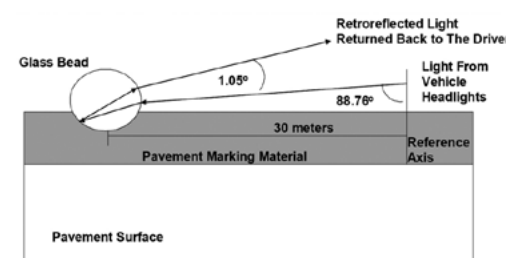
Fig. 3 Specification of retrorreflivity measurement
